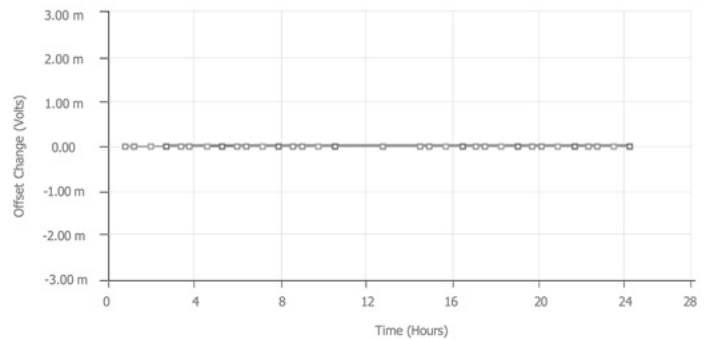
FIGURE 21 Voltage Drift with Self-Calibration
